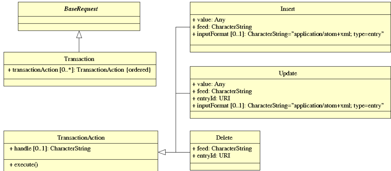
Figure 5 – Transaction UML class diagram
