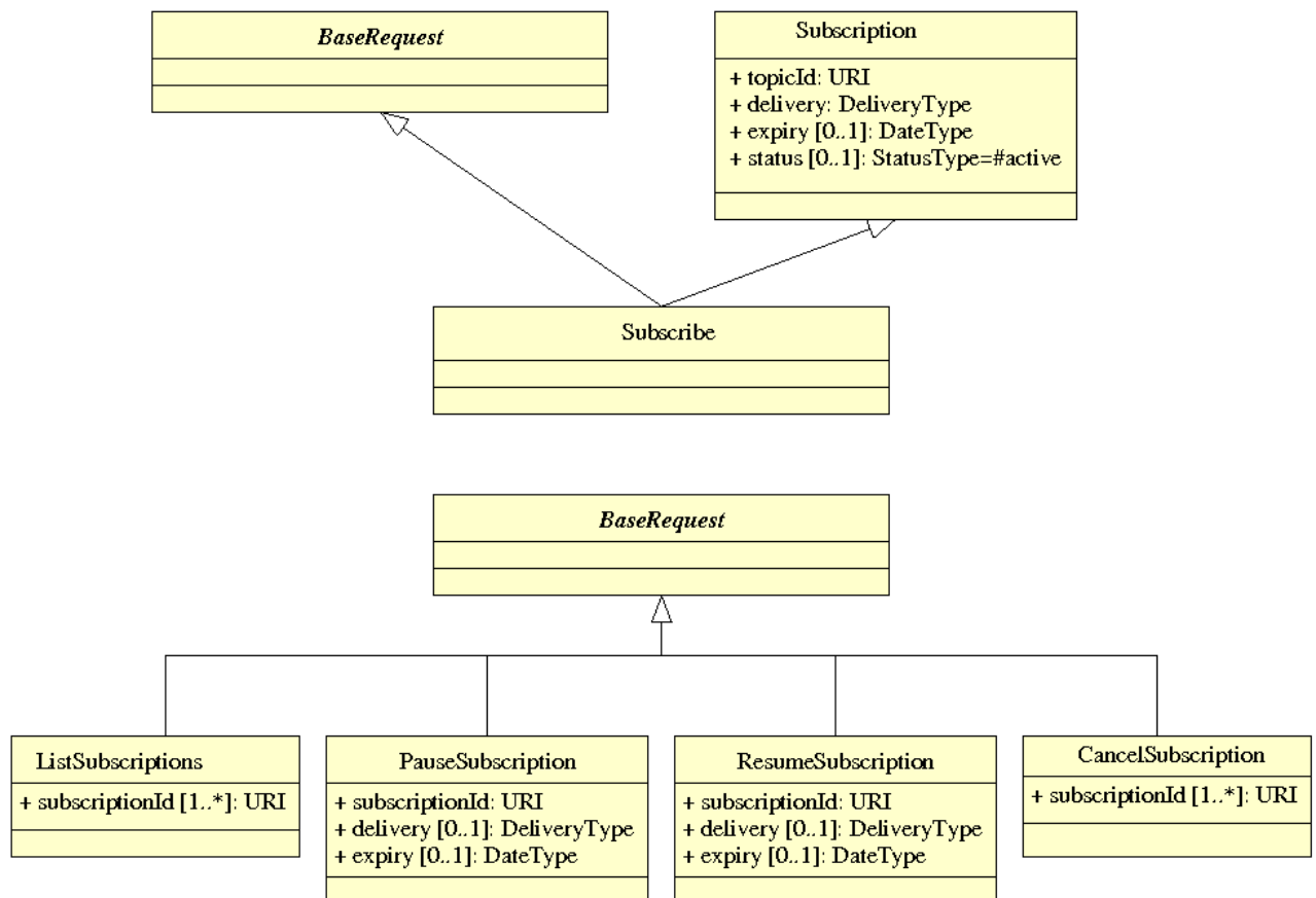
Figure 13 – Active notification UML class diagram
